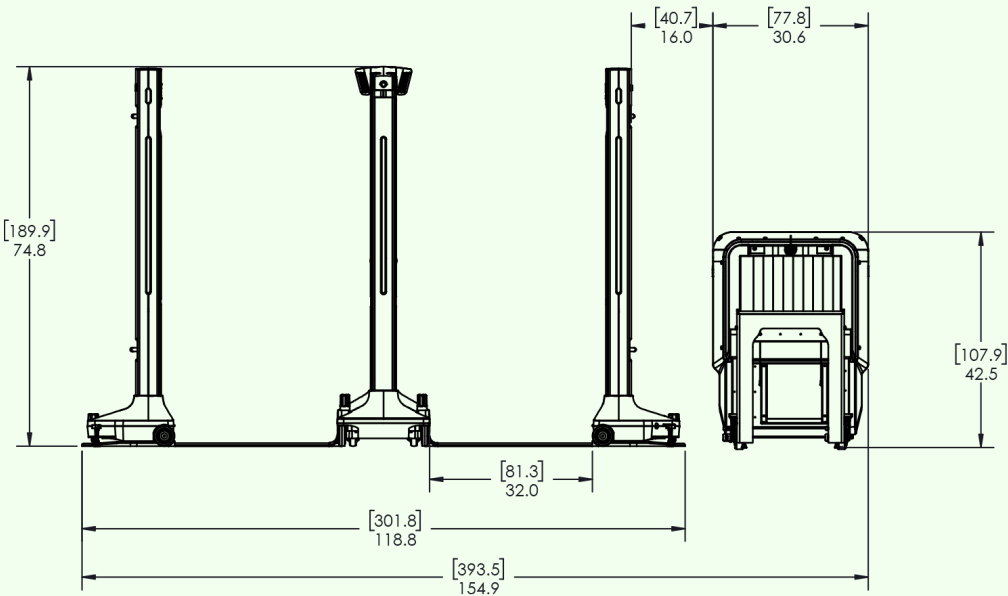
Front/Back View - Evolv eXpedite with Evolv Express Dual-Lane
