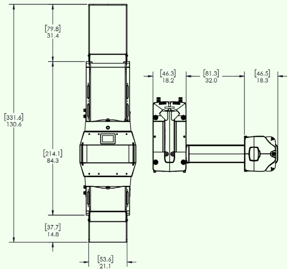
Top Down – Evolv eXpedite with Evolv Express Single-Lane
