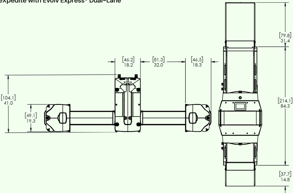
Top Down - Evolv eXpedite with Evolv Express® Dual-Lane
